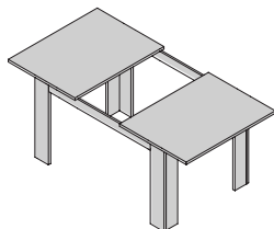
SR2-38 900x1350/1800x760
